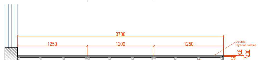
Townhall Stage SECTIONAL Details A preliminary for information
