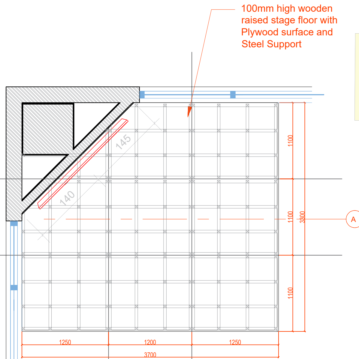
Townhall Stage Floor Plan Details
